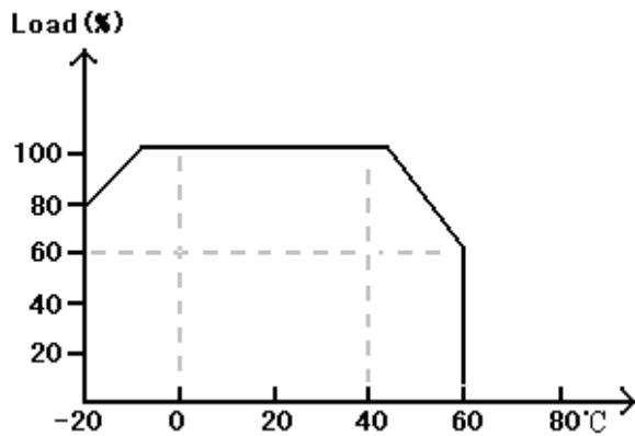
Temperature- load curve
